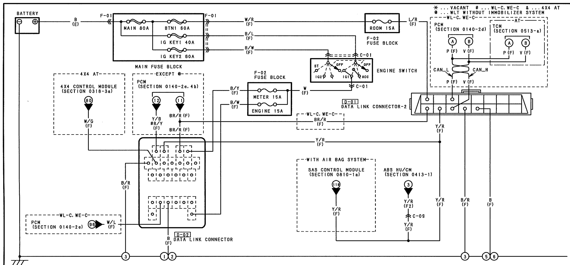
D-01 DATA LINK CONNECTOR-2 (F)
